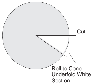
Atlas Forward LOX Tank Bulkhead (Cement to Card Stock)
