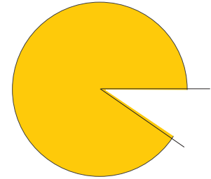
27. Gemini Adapter Module Aft Cover. Roll to Cone with Gold Side Pointing Inward. Cement Small Strip of Holding Paper on White Side. Gold Side Faces the Rear of Adapter Module*
