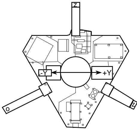
SPACECRAFT BUS TOP
